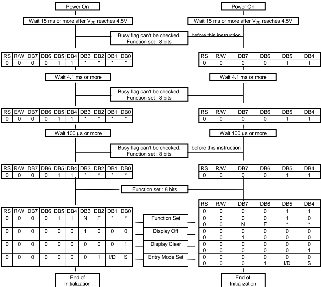
1) 8 Bit Interface
