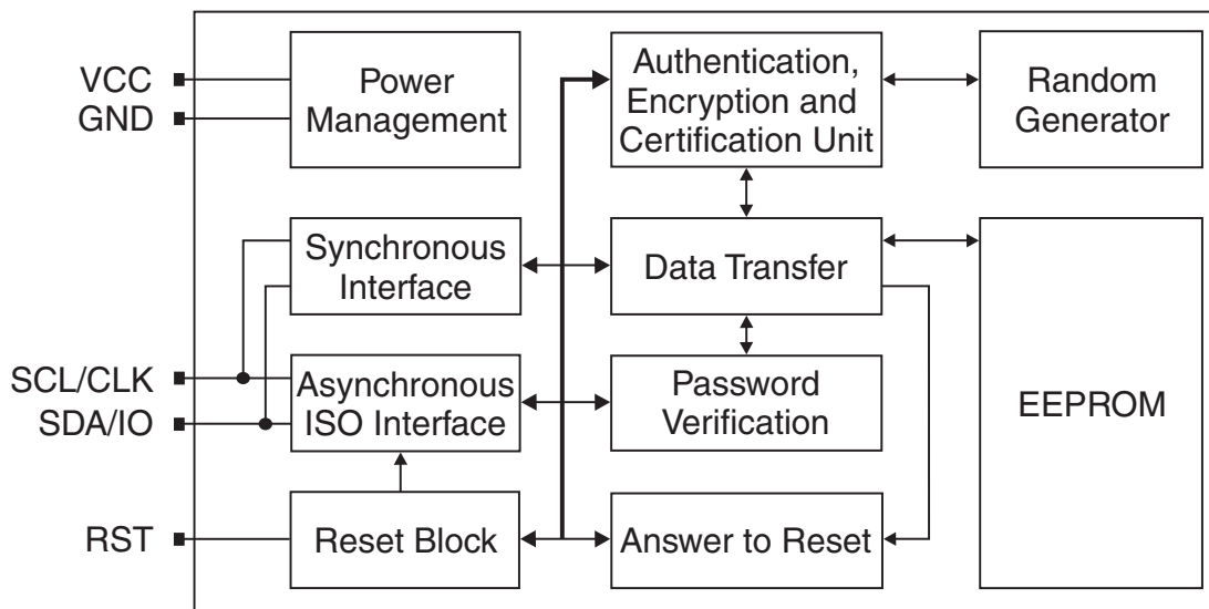
Figure 4-1. Block Diagram
