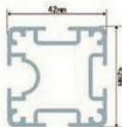
支架型材截面图 Sectional view of bracket
