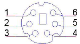
MINI-DIN 6Pin Female
