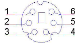
MINI-DIN 6Pin Male Contact side
