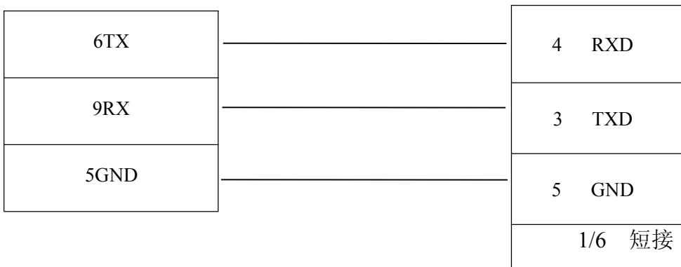
MINI-DIN 6Pin Female
