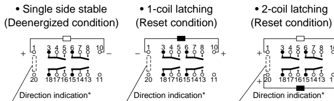
Schematic (Bottom view)
